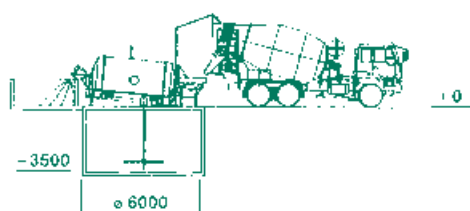
RA 12/20 installed over circular concrete basin
