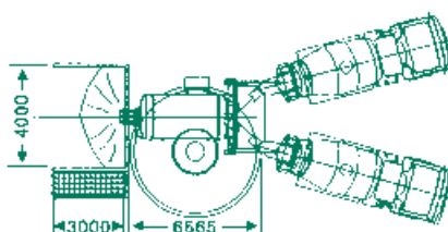
RA 12/20 installed over circular concrete basin
